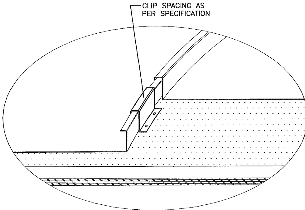
CLIP FASTENING SYSTEM
